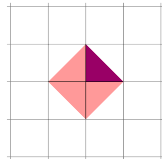
Figure 3.3: The orthoplex P_1 in \mathbb{R}^2 , dissected into 2^2 right triangles (one of which is shaded).
