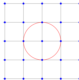
Figure 5.1: The lattice \mathcal{O}_F in blue dots, and the curve \lambda(\alpha) \in H in red. Here F = \mathbb{Q}(\sqrt{-1}) .
