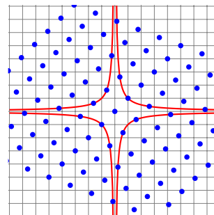
Figure 5.2: The lattice \mathcal{O}_F in blue dots, and the curve \lambda(\alpha) \in H in red. Here F = \mathbb{Q}(\sqrt{5}) .
